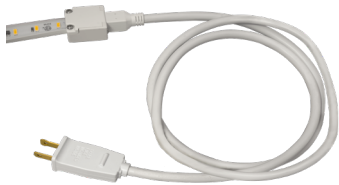
POWER FEED WITH 2-PRONG PLUG, 48IN (replaceable 5A fuse included in plug end)
