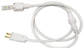
POWER FEED WITH 2-PRONG PLUG, 48IN (with connector for extending power feed runs, replaceable 5A fuse located in plug end)
