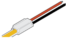
TAPE-TO-WIRE, 6IN WIRE COB CONNECTOR LLI-CB-CON-SC-10MM-6IN 6" wire included Connector: 0.53"L x 0.45"W x 0.15"H
