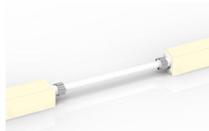
Jumper Power Connector (maximum 4 per run) SERIES SIDE LENGTH (L) LLI-NS3-68-CON2 — — SR 12IN SL 39IN EF 118IN RF 196IN 393IN
