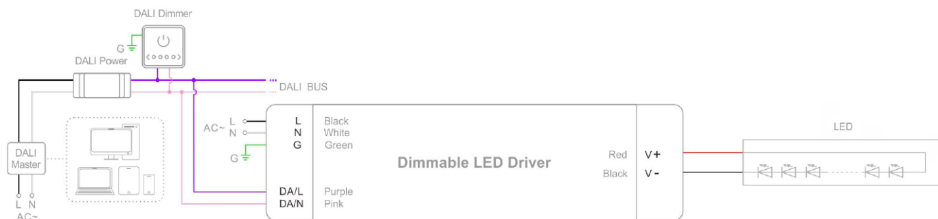
with intelligent device, DALI master, and DALI dimmer
