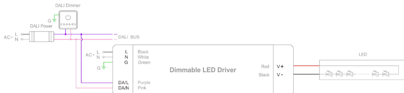
with DALI power and DALI dimmer
